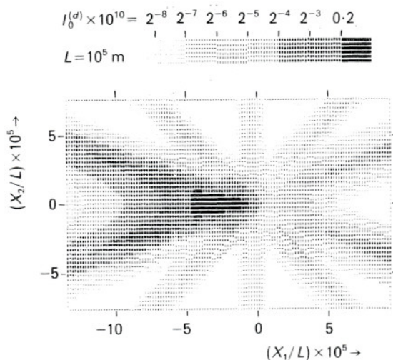
Fig. 4. The forward direct-beam topograph computed in the case of six-beam (220/242/044/224/202) diffraction of Cu K\alpha radiation in a Ge crystal of thickness 0.2 mm. The distance between the source and the film L = 10^5 m.
